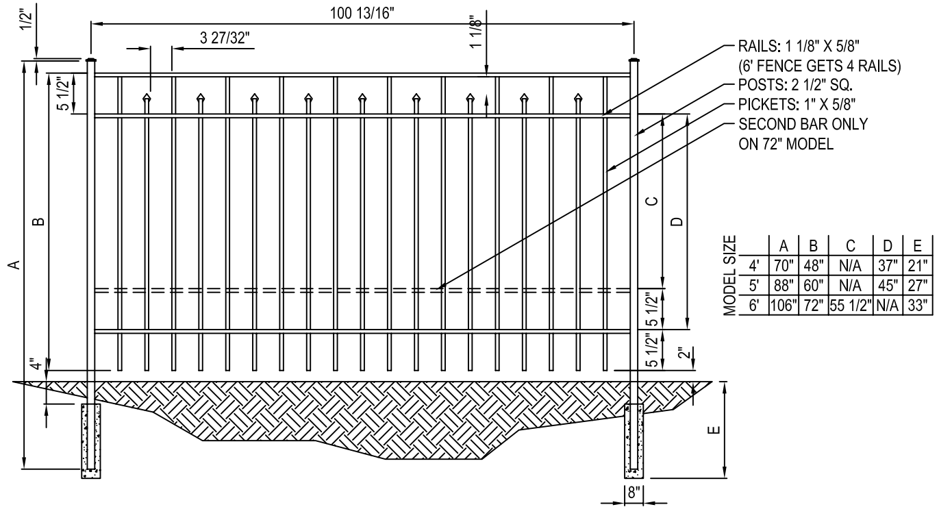
ELEVATION VIEW
